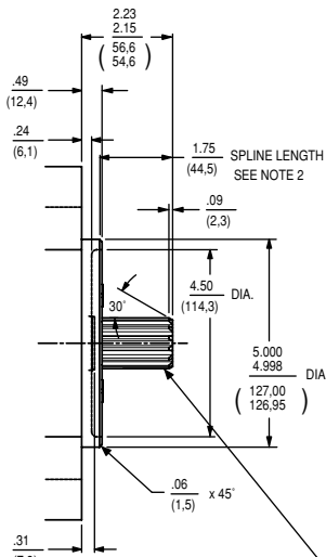
SAE 127-2 ("C" 2-BOLT) SAE 32-4 ("C" SPLINE)
