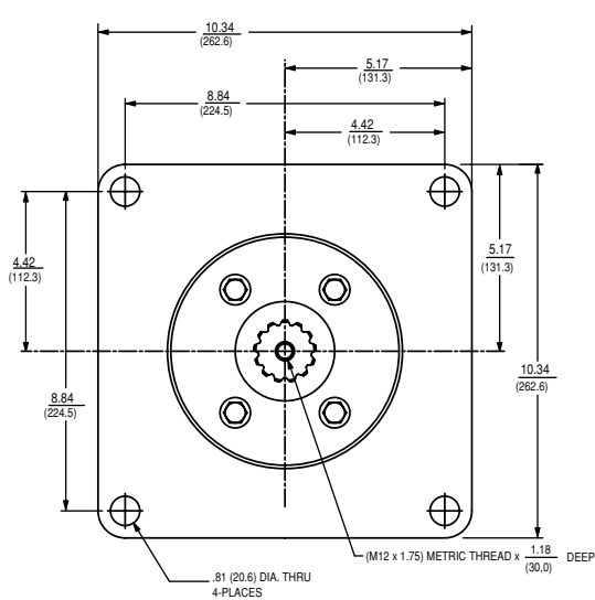
VIEW B-B
