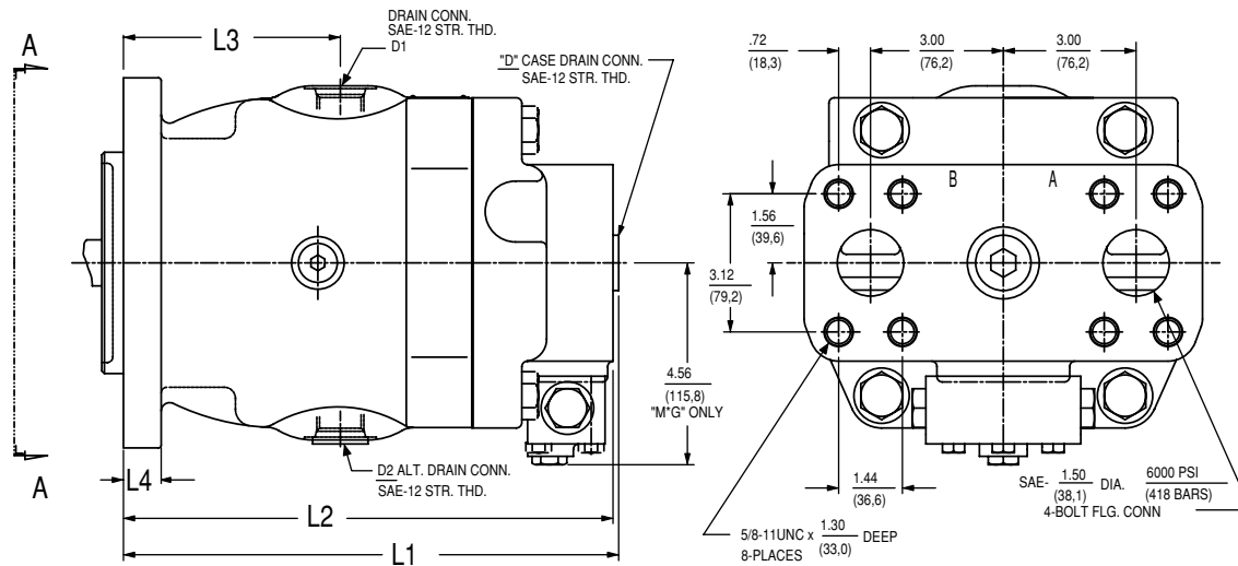
INSTALLATION DWG. 23-9294-D
