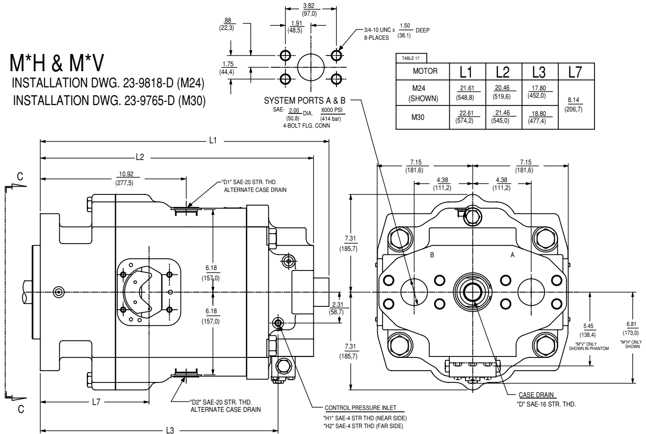
24-30 MOTOR DIMENSIONS (LESS CONTROLS)
