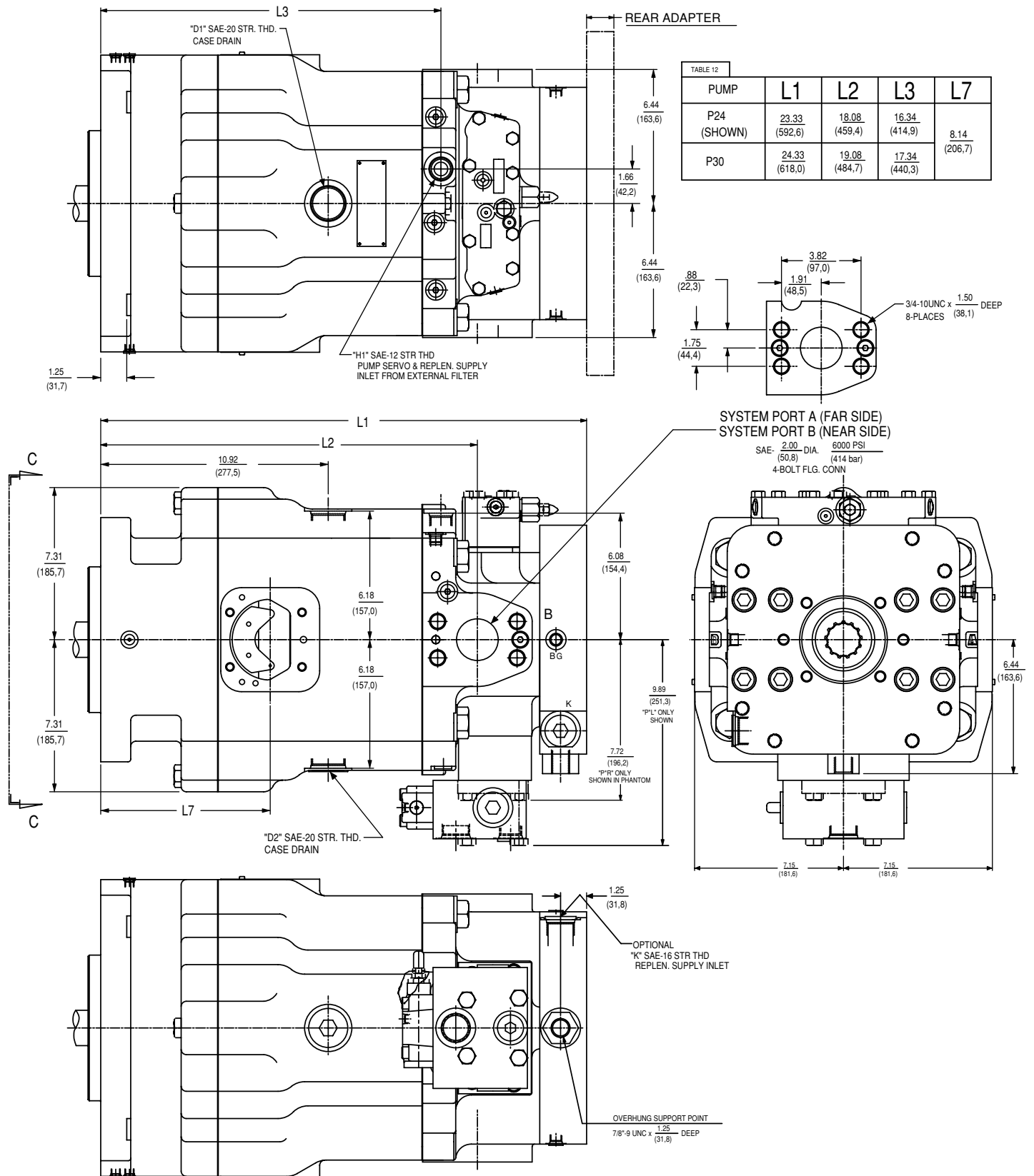
P*R & P*L INSTALLATION DWG. 23-10112-D
