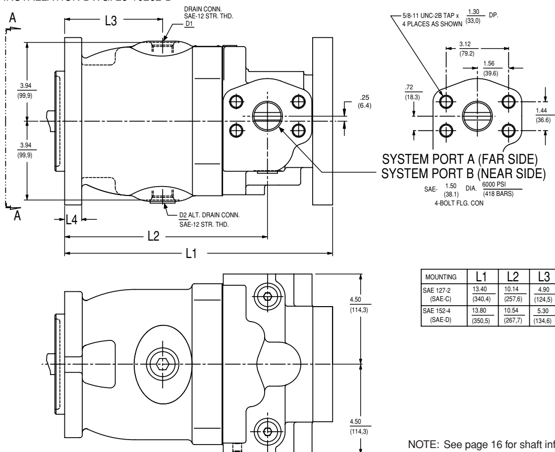
P*M INSTALLATION DWG. 23-10262-D
